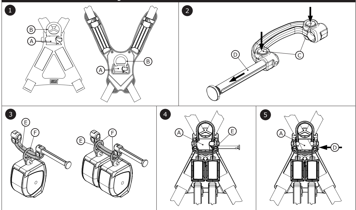
Figure 8A - Standard Harness Interface
