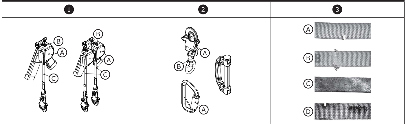
Figure 15 - Energy Absorber Pack Inspection
