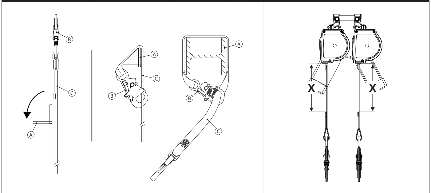
Figure 9 - Connecting to Anchorage Using Tie-Back Connectors
