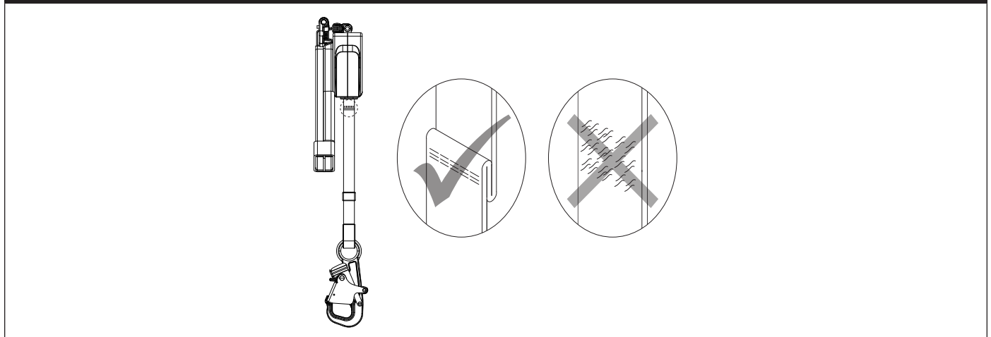
Figure 16 - Stitched Impact Indicator
