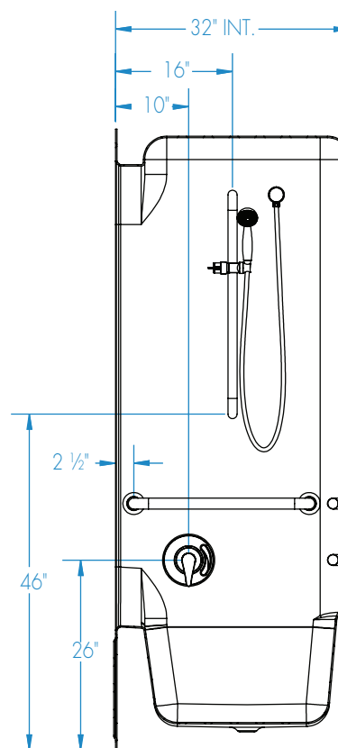
SECTION B-B
