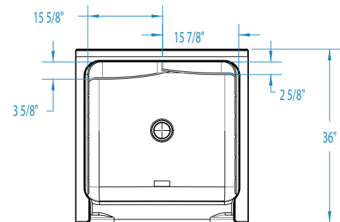
SECTION R-R
