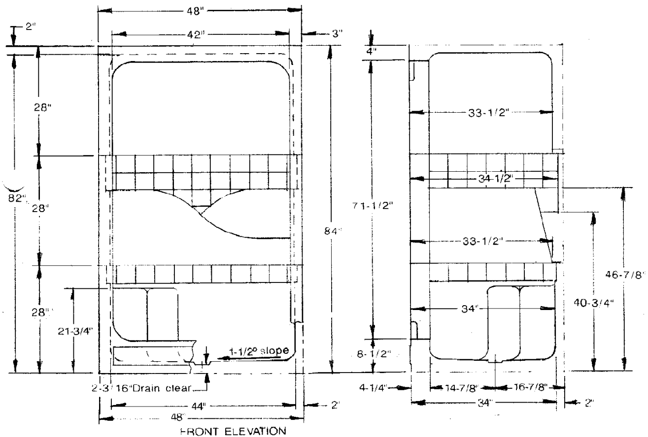
FRONT ELEVATION
