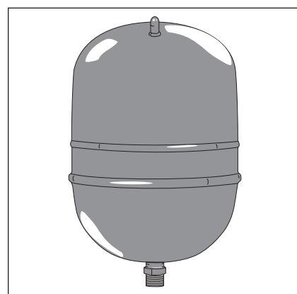
Figure 20 - The Thermal Expansion Tank should be pressurized with air to match the home's incoming water pressure.
