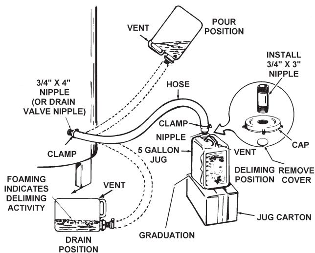
DELIMING THE COF WATER HEATER FIGURE 18
