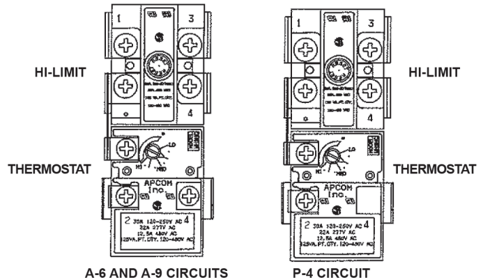
ADJUSTABLE UPPER THERMOSTAT BEHIND UPPER ACCESS PANEL
