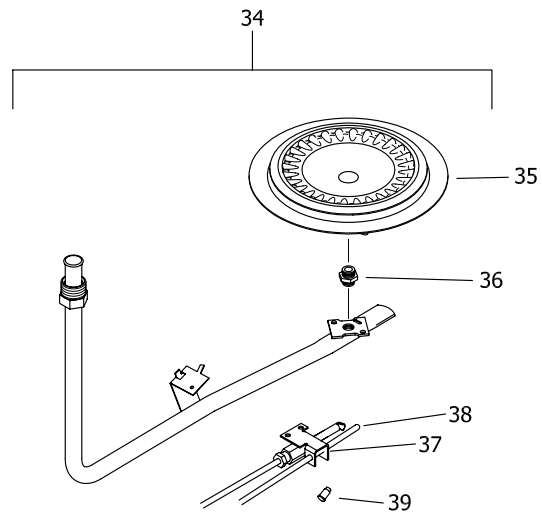
NATURAL GAS (BN) BURNER ASSEMBLY
