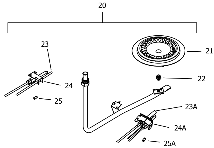
NATURAL GAS (BN) BURNER ASSEMBLY
