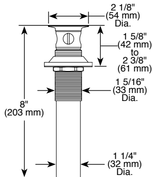
RP52487▲ Push Pop w/ Overflow Optional
