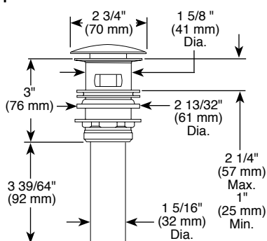
RP52487▲ Push Pop w/ Overflow Optional
