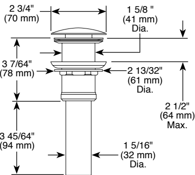
RP52488▲ Push Pop w/o Overflow Optional
