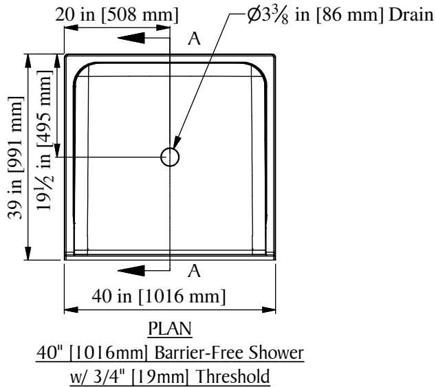
CENTER DRAIN
