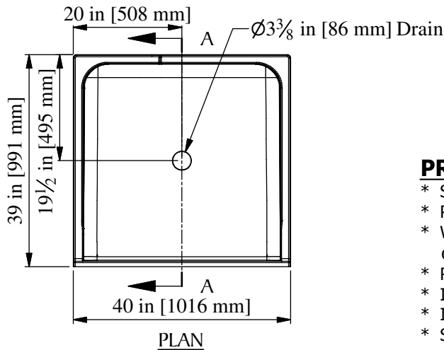
40" [1016mm] Barrier-Free Shower w/ 3/4" [19mm] Threshold
