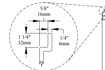
Close-up view of the nailing flanges on Clarion Bathware acrylic models
