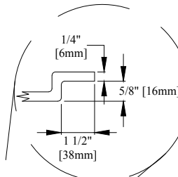
Close-up view of the nailing flanges on Clarion Bathware acrylic models
