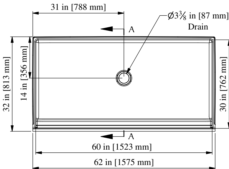
62" [1575mm] x 32" [813mm] Shower Pan w/ 3/4" [19mm] Threshold
