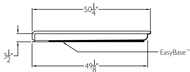
CROSS SECTION OF THRESHOLD
