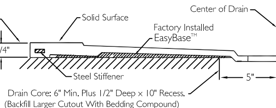
CROSS SECTION OF THRESHOLD
