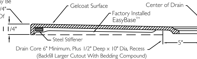
CROSS SECTION OF THRESHOLD
