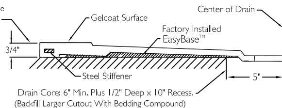
CROSS SECTION OF THRESHOLD
