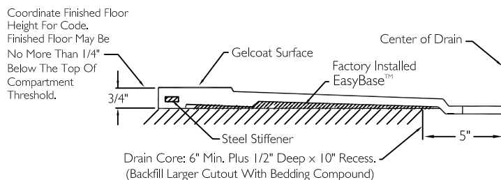
CROSS SECTION OF THRESHOLD
