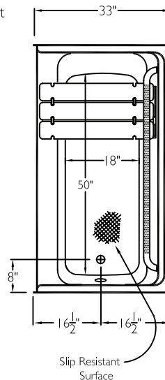
TOP VIEW
