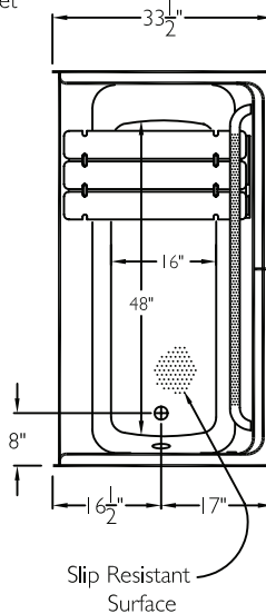
TOP VIEW
