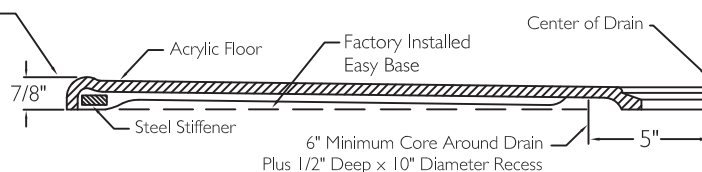
CROSS SECTION OF THRESHOLD
