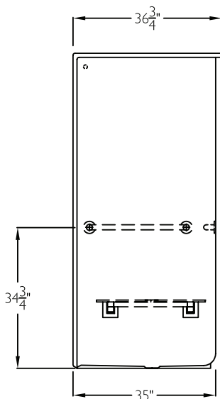
CROSS SECTION OF THRESHOLD
