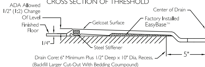
CROSS SECTION OF THRESHOLD
