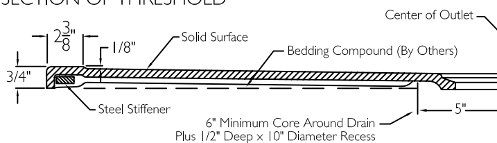
CROSS SECTION OF THRESHOLD
