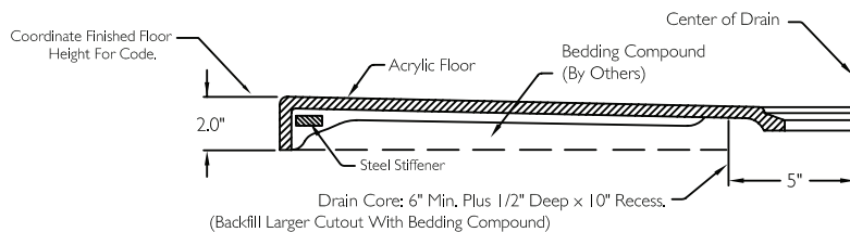
CROSS SECTION OF THRESHOLD
