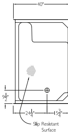
TOP VIEW
