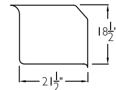
SEAT DIMENSIONS
