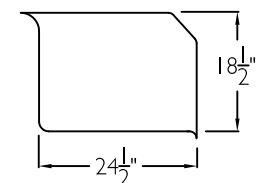
SEAT DIMENSIONS
