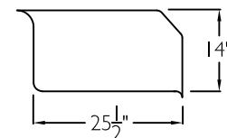
SEAT DIMENSIONS
