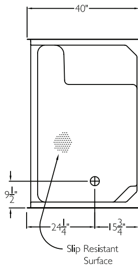
TOP VIEW
