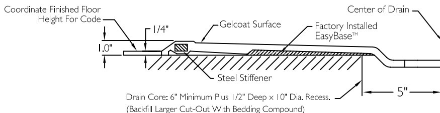
CROSS SECTION OF THRESHOLD
