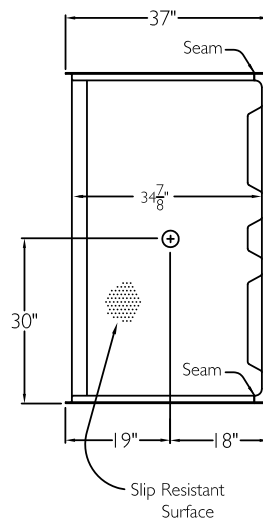
TOP VIEW
