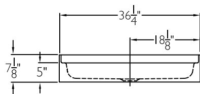
ENTRY END VIEW
