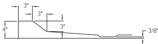
MODIFIED THRESHOLD DETAIL
