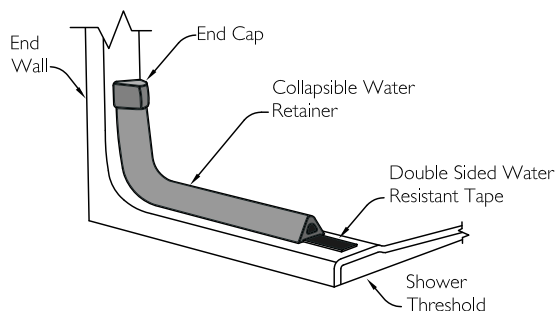
Showers With Large Corner Radius
