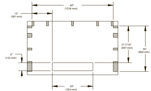
TRENCH DRAIN CUTAWAY & STUD PLACEMENT
