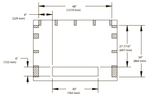
TRENCH DRAIN CUTAWAY & STUD PLACEMENT
