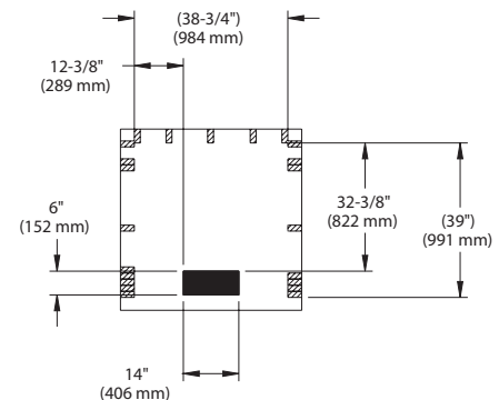
TRENCH DRAIN CUTAWAY & STUD PLACEMENT
