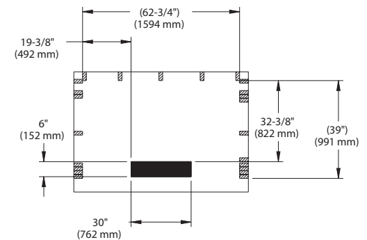
TRENCH DRAIN CUTAWAY & STUD PLACEMENT
