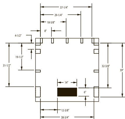
TRENCH DRAIN CUTAWAY & STUD PLACEMENT
