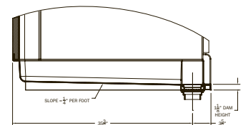
DETAIL VIEW
