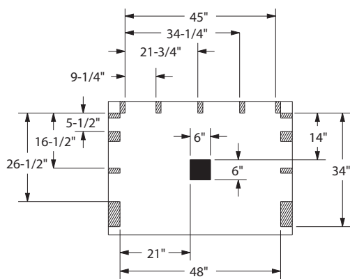
TRENCH DRAIN CUTAWAY & STUD PLACEMENT
