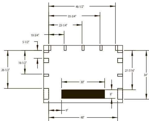
TRENCH DRAIN CUTAWAY & STUD PLACEMENT
