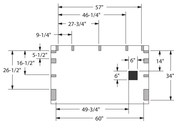
TRENCH DRAIN CUTAWAY & STUD PLACEMENT
