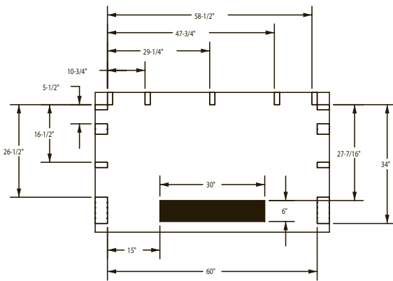
TRENCH DRAIN CUTAWAY & STUD PLACEMENT
