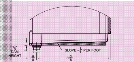
DETAIL VIEW
