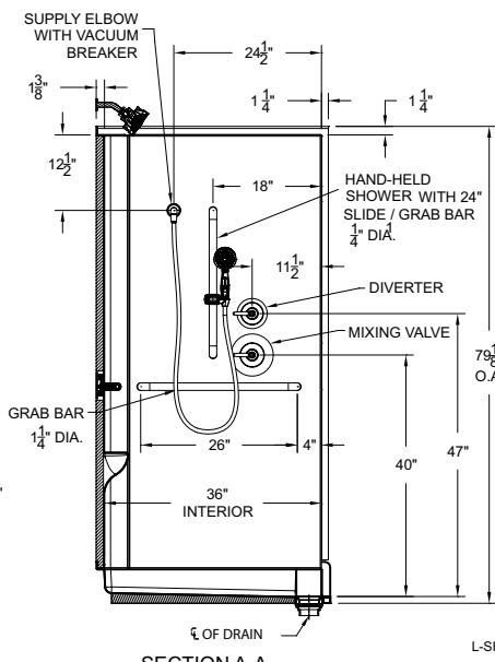
SECTION A-A SIDE VIEW
