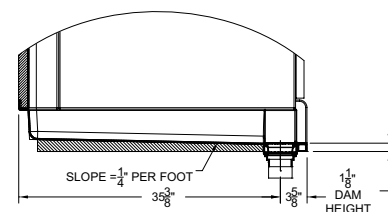
DETAIL VIEW
