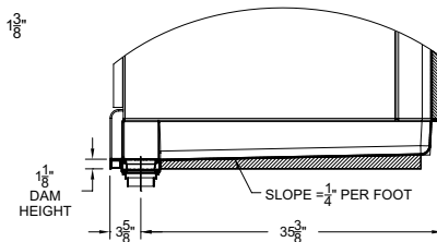
DETAIL VIEW
