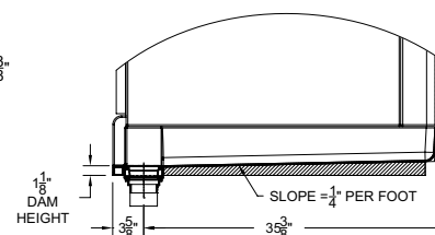
DETAIL VIEW
